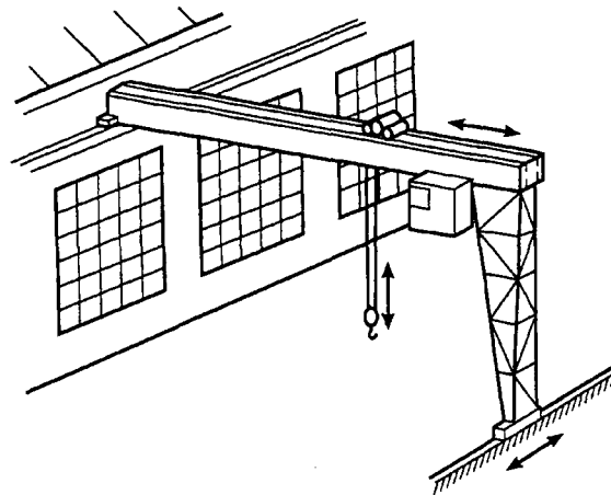
FIG. 4 SEMIGANTRY CRANE
